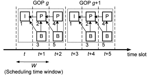
Fig. 2. Illustration of GOP (group of pictures), DU (data unit), and the context. Since the scheduling time window is W = 2 , the contexts in different time slots are C_t = \{DU_1^g, DU_2^g, DU_3^g\} , C_{t+1} = \{DU_2^g, DU_3^g, DU_4^g, DU_5^g\} , C_{t+2} = \{DU_4^g, DU_5^g, DU_1^{g+1}\} , C_{t+3} = \{DU_1^{g+1}, DU_2^{g+1}, DU_3^{g+1}\} , and so on.
