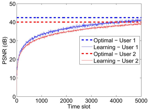
Fig. 5. Convergence of the PDS-based learning algorithm.
